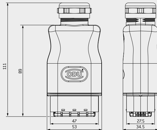
PLUG
