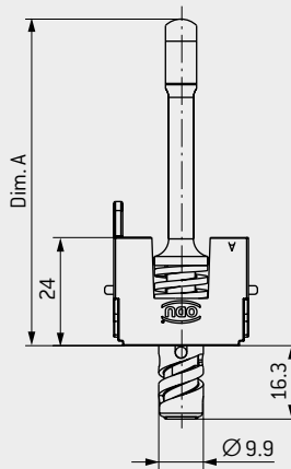
SPINDLE 3 – 16.3 mm (360°)
