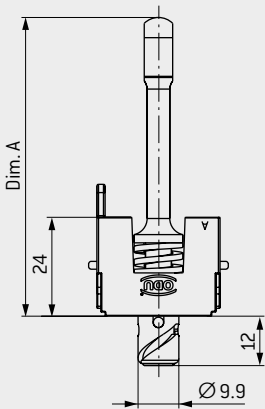
SPINDLE 1 – 12 mm (180°)
