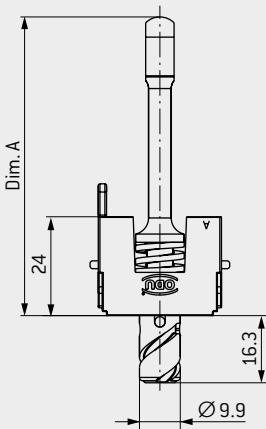
SPINDLE 2 – 16.3 mm (270°)
