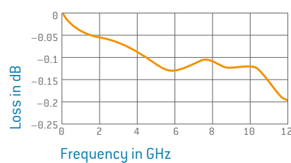
Insertion loss
