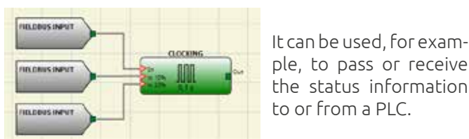
Clocking operator connection sample
