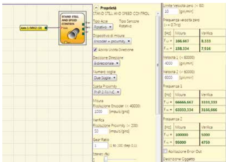
Speed monitoring object configuration example
